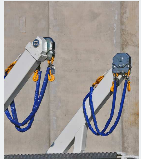
Loadcells mounted at end of lifting arms with chains for bin
